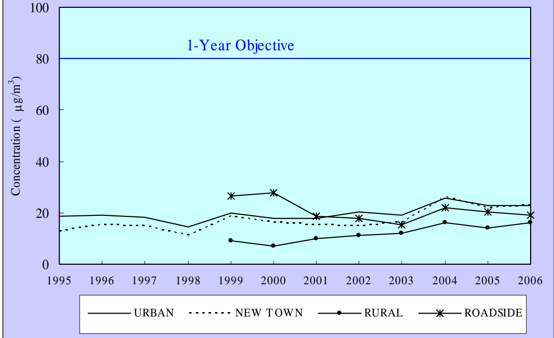
Figure 2 : Sulphur Dioxide (SO 2 ) long term trend
