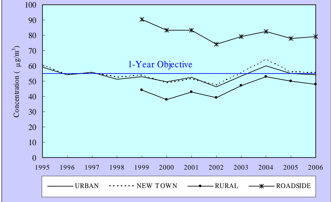
Figure 1 : RSP (PM10) long term trend
