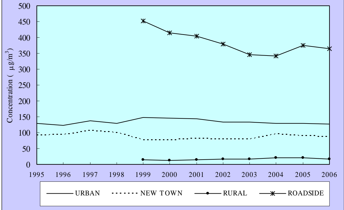
Figure 4 : Nitrogen Oxides (NO x ) long term trend
