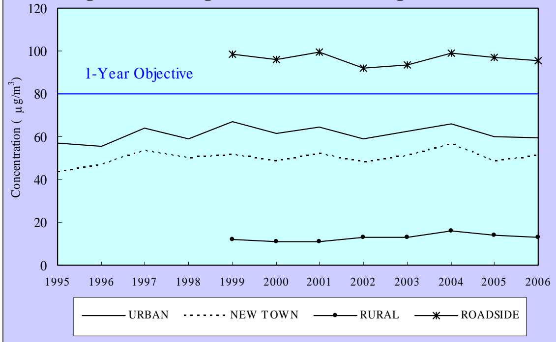
Figure 5 : Nitrogen Dioxide (NO 2 ) long term trend
