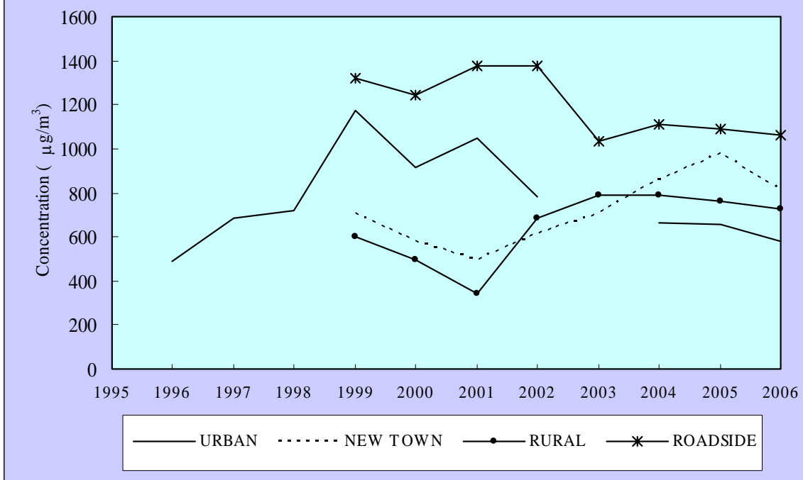
Figure 6 : Carbon Monoxide (CO) long term trend
