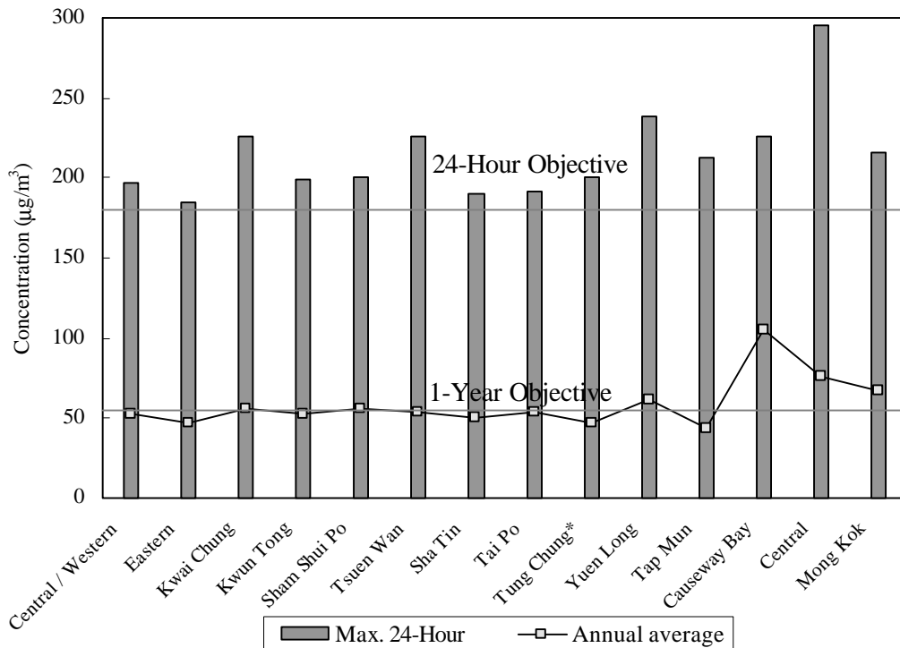
Figure 7: RSP Monitoring 1999
