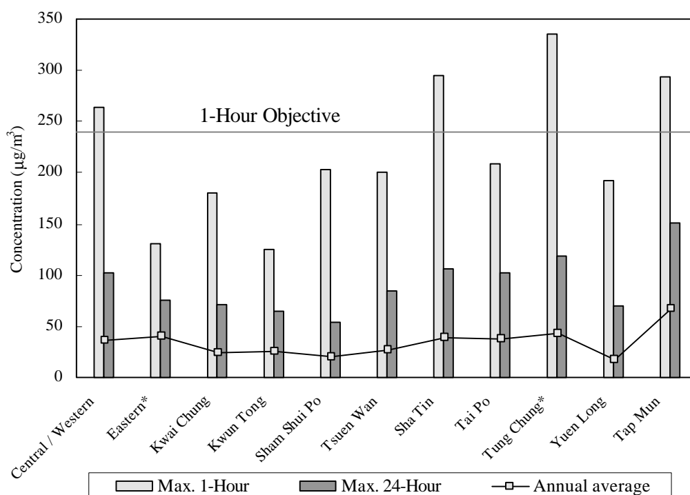
Figure 4: Ozone Monitoring 1999
