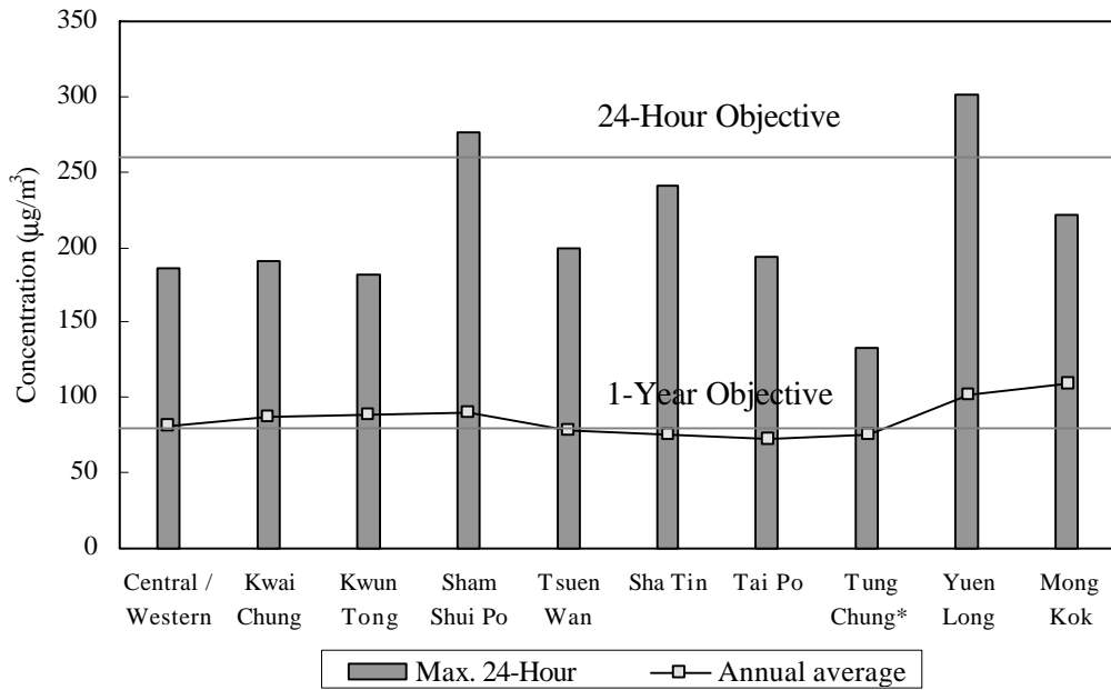
Figure 6: TSP Monitoring 1999
